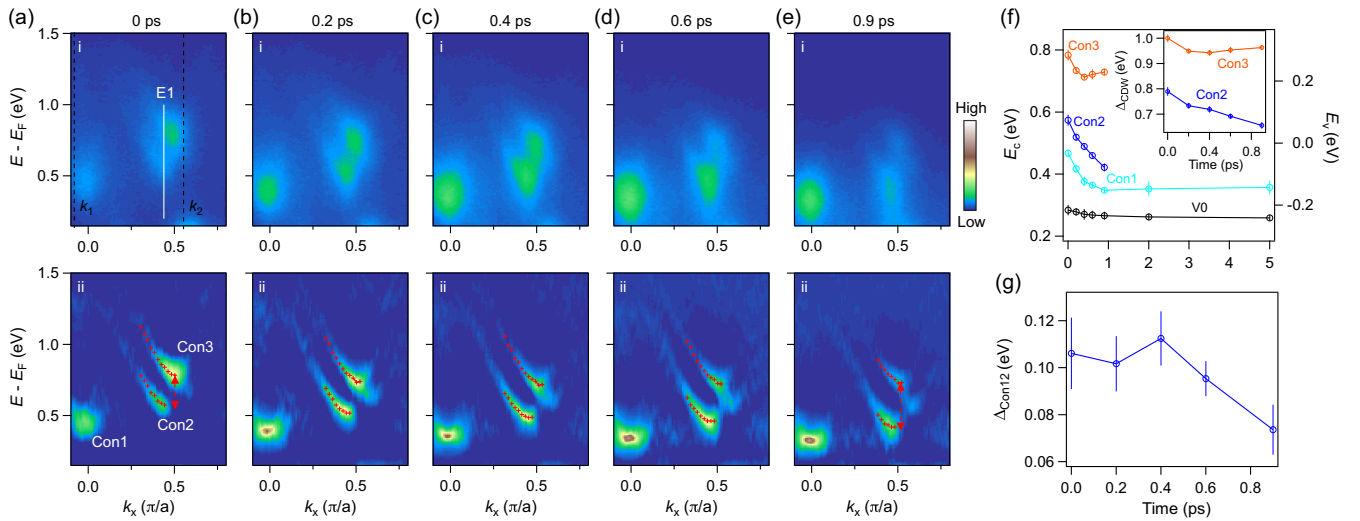
FIG. 3. Temporal evolution of conduction bands and CDW gaps. (a)–(e) ARPES (i) and curvature (ii) intensity plots along the C1 direction at t = 0, 0.2, 0.4, 0.6, and 0.9 ps, respectively. The red symbols are peak positions of Con2 and Con3 bands, obtained from the Lorentzian fitting of the energy distribution curves at each k_x point and at each delay time. (f) Extracted time-dependent conduction band bottoms. The inset shows the corresponding CDW gaps determined from the difference between the bottom of Con2 or Con3 and the top of V0. (g) Time-dependent band-bottom difference of Con1 and Con2. The error bars represent the statistical uncertainty derived from the fitting procedure.
