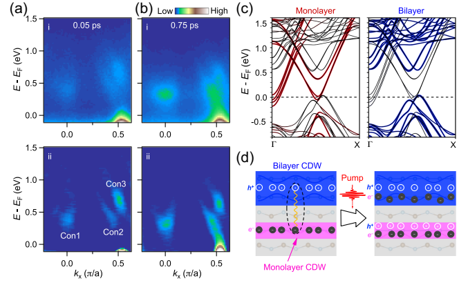
FIG. 4. The interplay of intertwined CDW states. (a),(b) ARPES (i) and curvature (ii) intensity plots along the k_x direction at t = 0.05 and 0.75 ps, respectively. The pump fluence was 1.2 \text{ mJ/cm}^2 . (c) The calculated band structure along the \Gamma -X direction based on the (1 \times 3 \times 2) superlattice and the GGA type of the exchange-correlation potential. The red and blue colors represent the weight of p_x and p_y orbitals from the Te monolayer and bilayer, respectively. (d) Schematic of the electron-hole interactions between CDWs residing in the monolayer and bilayer Te sheets. The white circles and black dots represent the holes and electrons, respectively. The orange curves denote the interactions, and the black-dotted ellipse represents an electron-hole pair.
