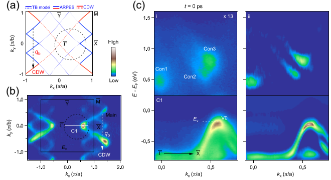
FIG. 2. Electronic structure and intrinsic CDW gaps of \text{EuTe}_4 . (a) Original (blue curves) and folded (red curves) Fermi surface based on tight-binding calculations. The solid lines represent the observed bands at E_v [shown in panel (b)]. The black dashed circle indicates the detection area of our tr-ARPES measurements. (b) ARPES constant energy map at E_v , measured with 90 eV, right circularly polarized light. (c) ARPES (i) and curvature (ii) intensity plots along the C1 direction [labeled in panel (b)], measured at t = 0 ps. The probe photon energy was 10.75 eV, and polarization was linear horizontal (LH, perpendicular to the photoemission plane). The pump photon energy was 1.55 eV, the polarization was LH, and the fluence was 0.16 \text{ mJ/cm}^2 .
