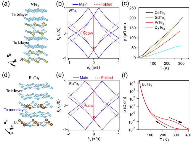
FIG. 1. Comparison between charge density waves in R\text{Te}_3 and \text{EuTe}_4 . (a) Crystal structure of R\text{Te}_3 , featuring Te bilayers whose states are closest to the Fermi level. (b) Calculated normal-state FS (blue lines) of R\text{Te}_3 based on the tight-binding model. The blue solid and red dashed lines represent the original and folded bands, respectively. Note that only parts of the folded bands are plotted for clarity. (c) Temperature-dependent electrical resistivity of R\text{Te}_3 , showing metallic behavior in the CDW state. The CDW transition temperatures of all the compounds shown are above 300 K. (d) Crystal structure of \text{EuTe}_4 . (e) Tight-binding normal-state FS of \text{EuTe}_4 , following the same convention as in panel (b). (f) Temperature-dependent electrical resistivity of \text{EuTe}_4 in the CDW state, showing semiconducting behavior and a giant thermal hysteresis. Panels (c) and (f) are extracted from Refs. [12] and [13], respectively.
